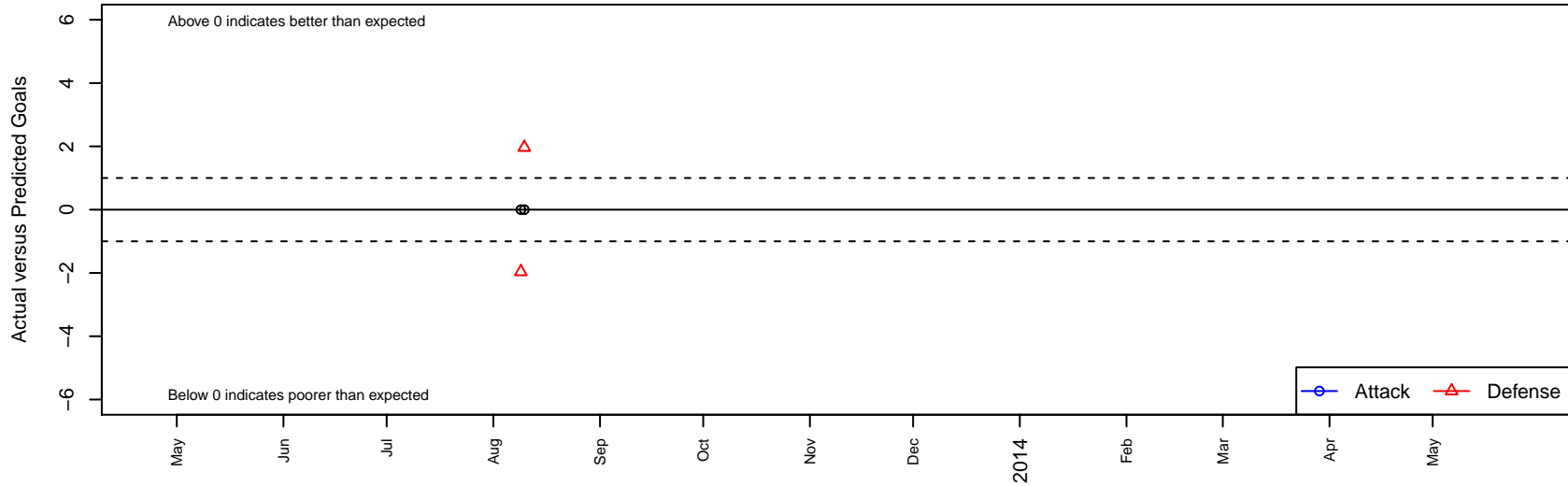
SGESC Explosion G99 Dots are actual minus expected GF (blue circles) and GA (red triangles). Blue line is smoothed change in attack strength. Red is smoothed change in defense strength.
